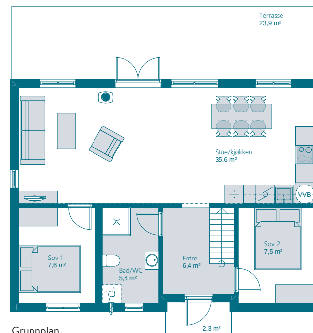
Grunnplan
